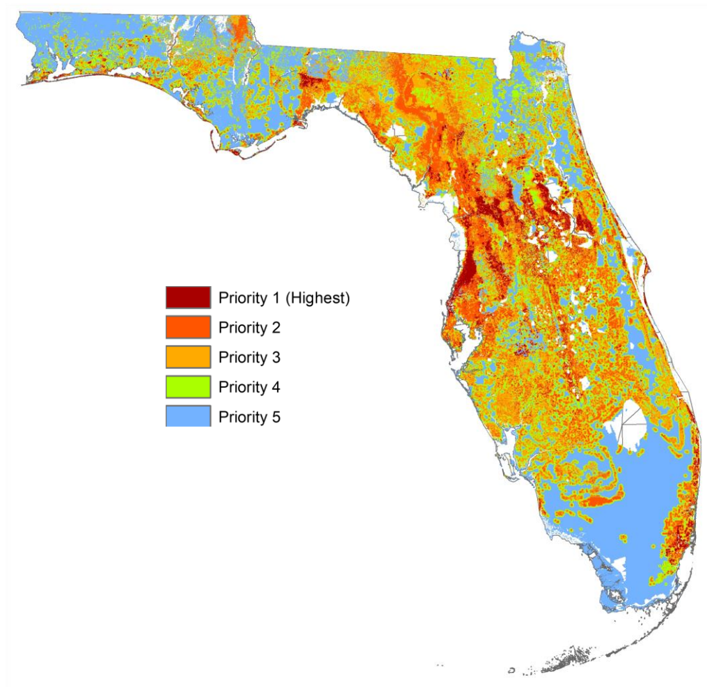
Figure 10-2. Five-class potential recharge model with discharge removed.
