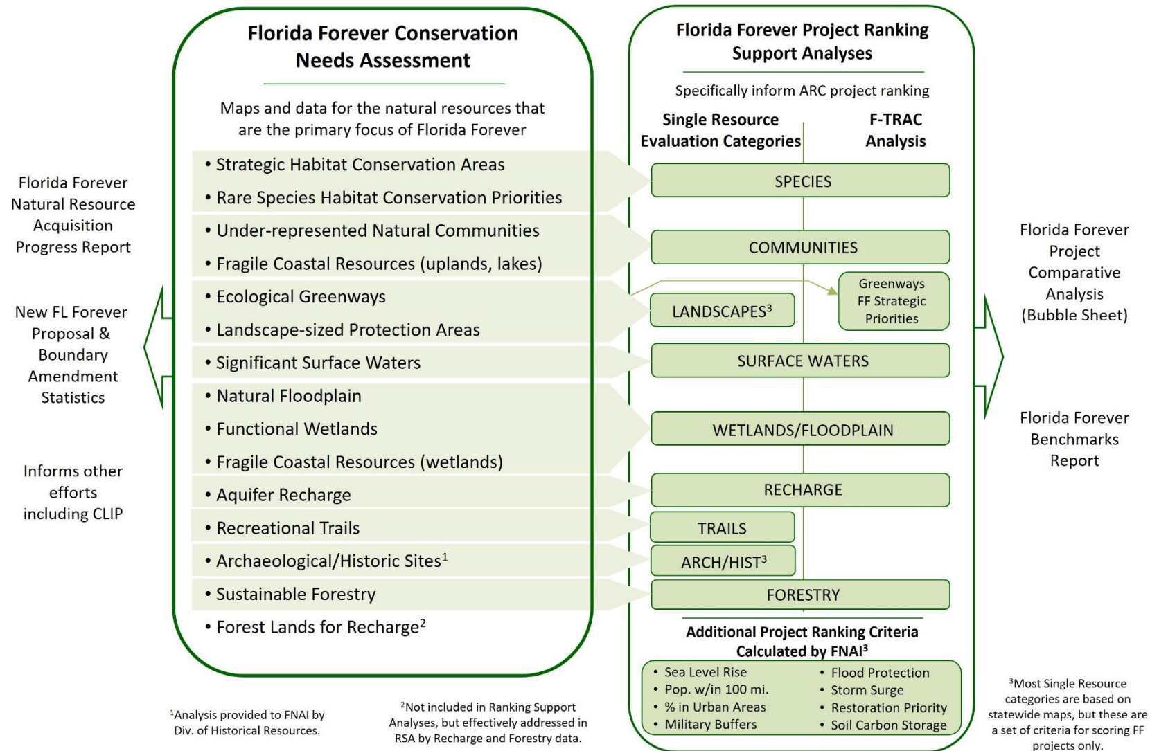
Figure 2. Relationships between Florida Forever data and analyses developed and maintained by Florida Natural Areas Inventory.
